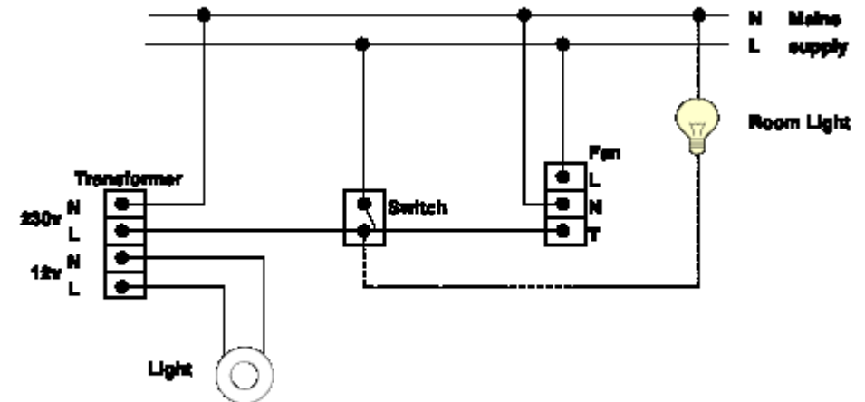
B: LuxVentT Plus - fans with overrun timer
